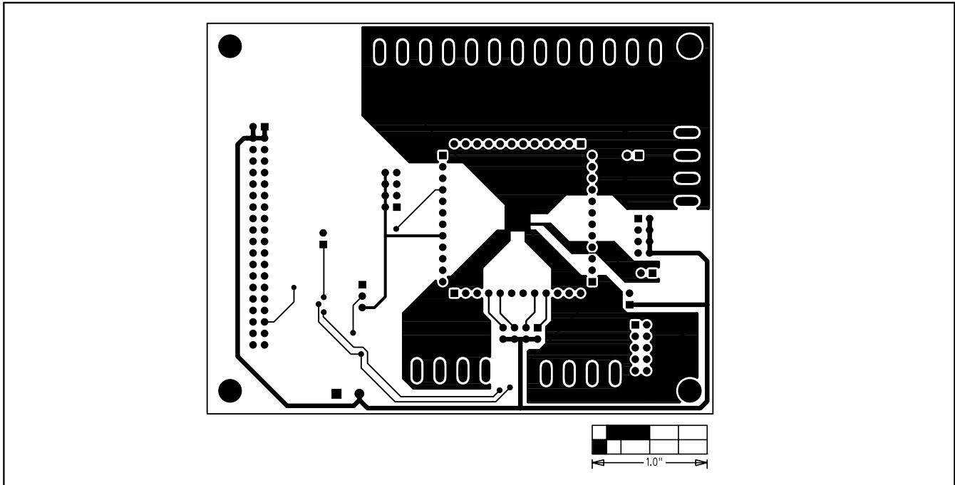
Figure 10. MAX1258 EV Kit PC Board Layout—Solder Side
