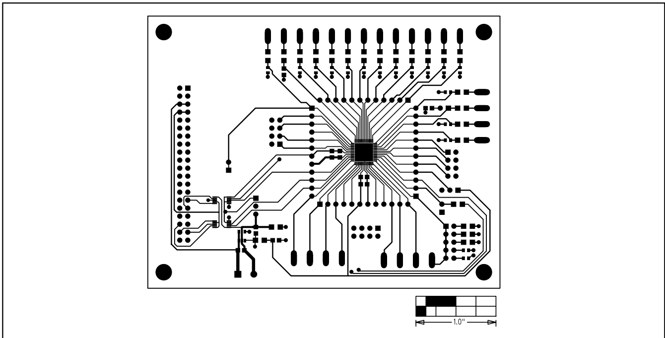
Figure 9. MAX1258 EV Kit PC Board Layout—Component Side
